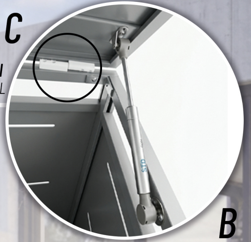
B ÜST KAPAK AÇILMA MEKANİZMASI GAZLI PİSTON TOP LID OPENING MECHANISM GAS STRUT
