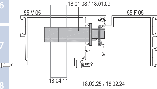
**İÇE AÇILIM HEMYÜZ DETAY İÇİN **INWARD OPENING FLUSH DOOR DETAIL
