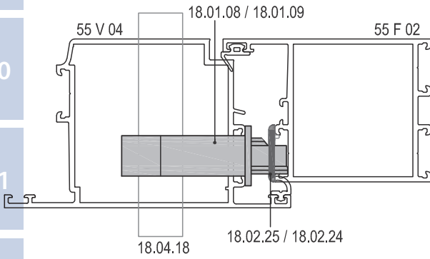
**DIŞA AÇILIM BİNLİ DETAY İÇİN **OUTWARD OPENING DOOR DETAIL
