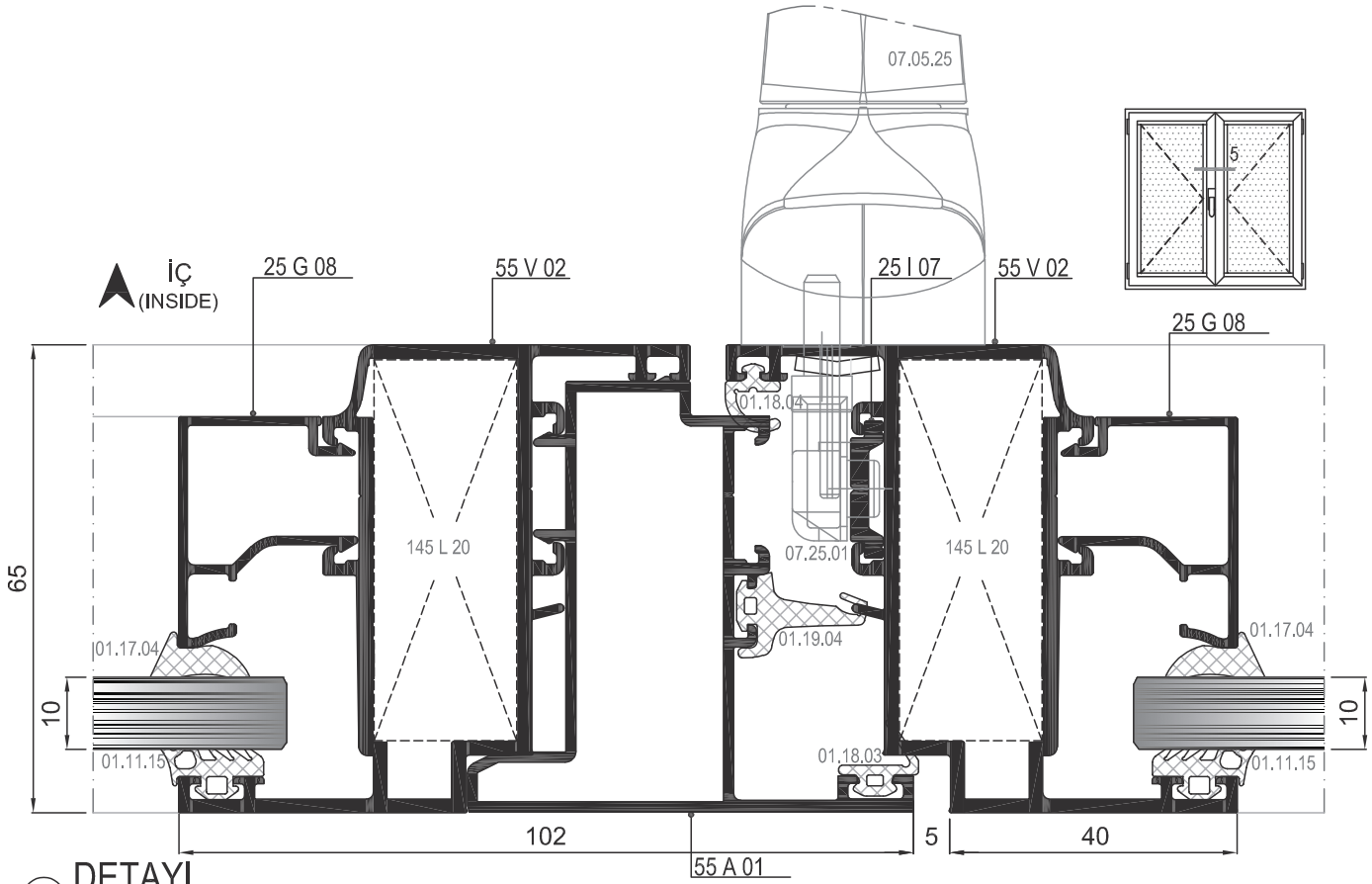
⑤ DETAYI DETAIL
