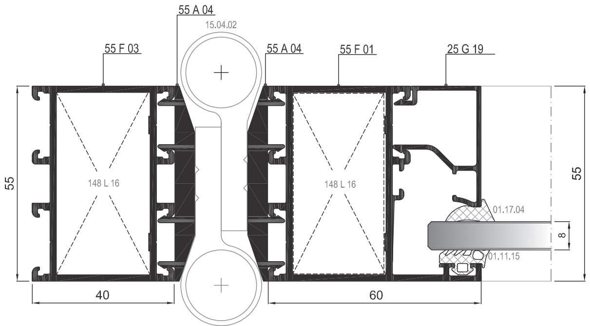
14 DETAYI DETAIL
